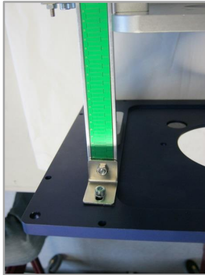
Mounting of the measuring scale on the underside of the inlay plate.
