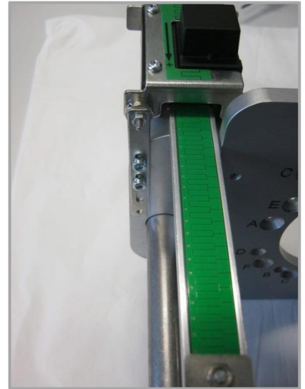
Mounting of the measuring scale on the underside of the inlay plate.
